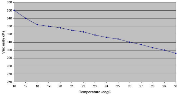
Viscosity Change with Temperature - APL
